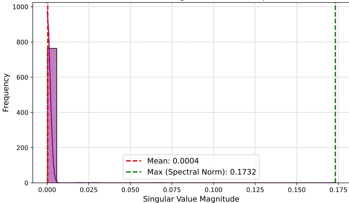
Distribution of Singular Values at Step 75
